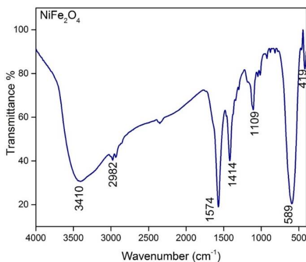
FIG. 2. FTIR spectra of \text{NiFe}_2\text{O}_4 .
